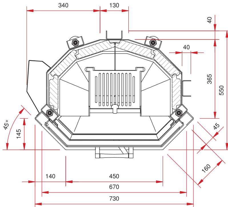
Top view M 1:10
