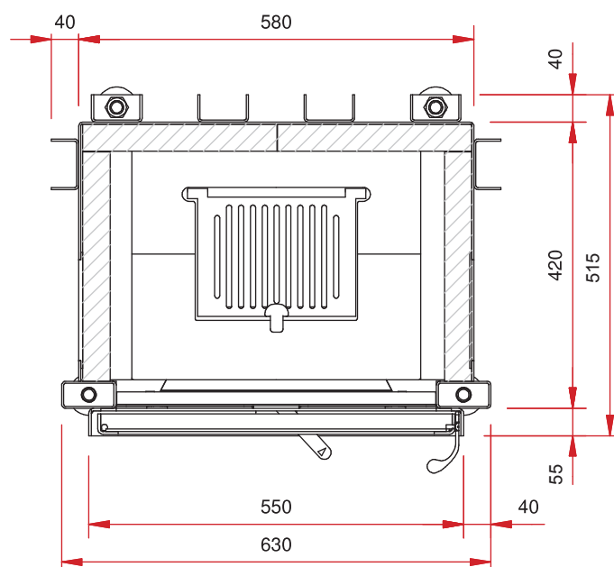
Top view M 1:10
